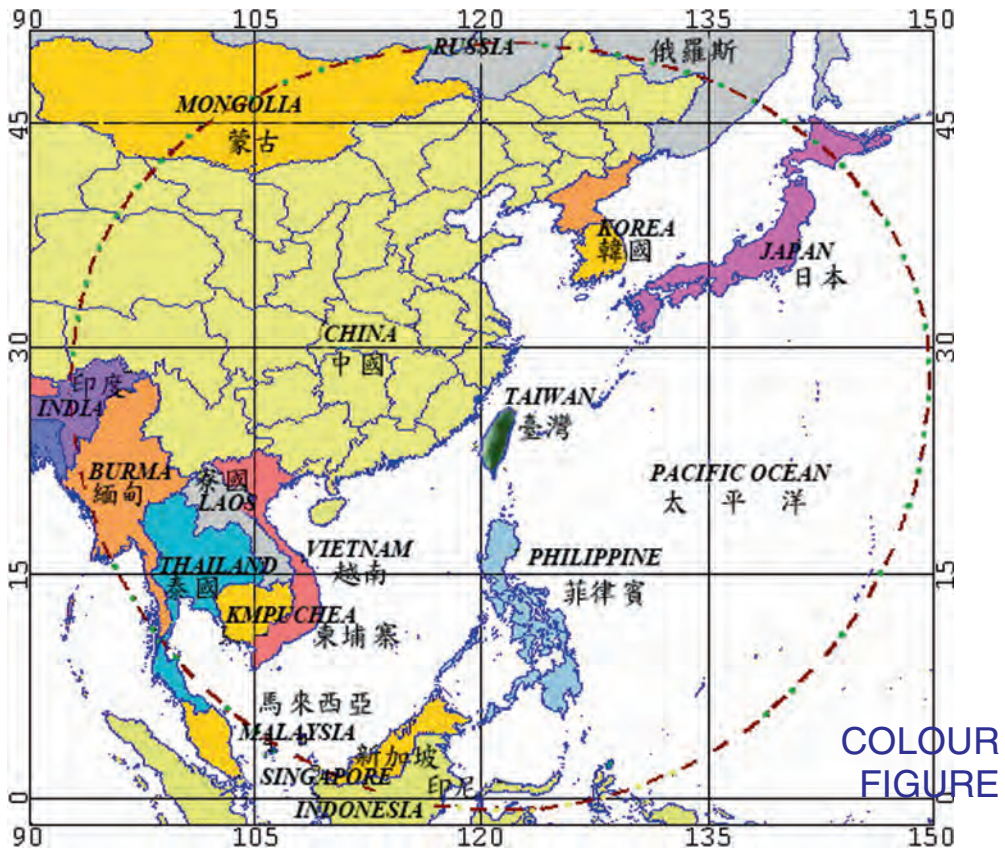
Figure 1. Reception zone of the Center for Space and Remote Sensing Research (CSRSR) receiving station ( http://www.csr.r.ncu.edu.tw ) covering an area of radius 3000 km; east of USA's Guam, west of China's Gang-Su, north of Japan's Hokkaido and south of the South China Sea.
