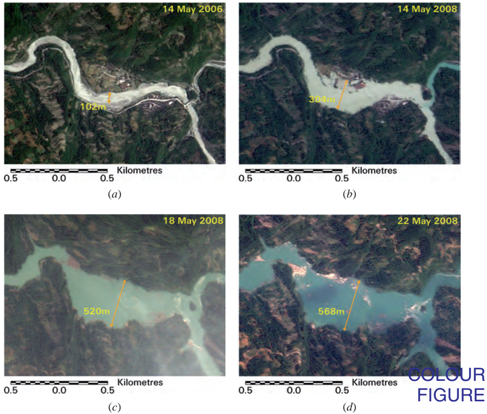
Figure 5. Successive FORMOSAT-2 satellite images of the pre- and post-earthquake situations of the river under study. (a) Pre-earthquake image taken on 14 May 2006, (b), (c), (d) successive post-earthquake images taken after 2 days, 6 days and 10 days, respectively from the date of the earthquake.
