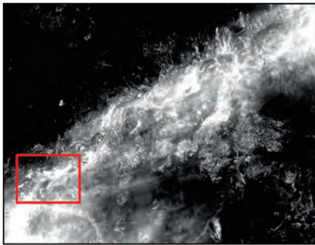
Figure 7. FORMOSAT-2 satellite image over-passing Wenchuan County at 11:46:35 am on 15 May 2008.
