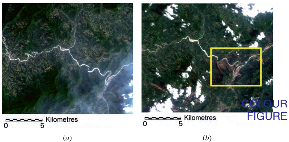
Figure 3. Satellite images of the affected area taken on 14 May 2008 (a) well before the earthquake and (b) immediately after the earthquake.
