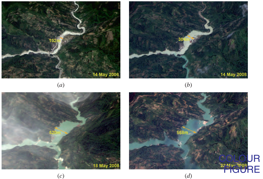
Figure 6. Successive 3-dimensional simulation with FORMOSAT-2 satellite images of the pre- and post-earthquake situation of the river under study. (a) Pre-earthquake image taken on 14 May 2006, (b), (c), (d) successive post-earthquake images taken after 2 days, 6 days and 10 days, respectively from the date of the earthquake.
